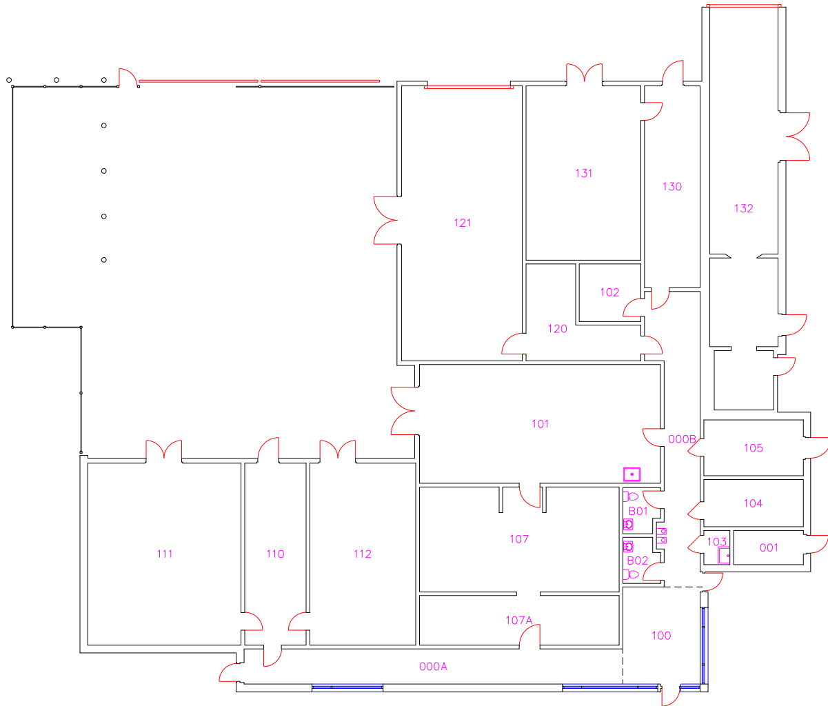
FIRST FLOOR
