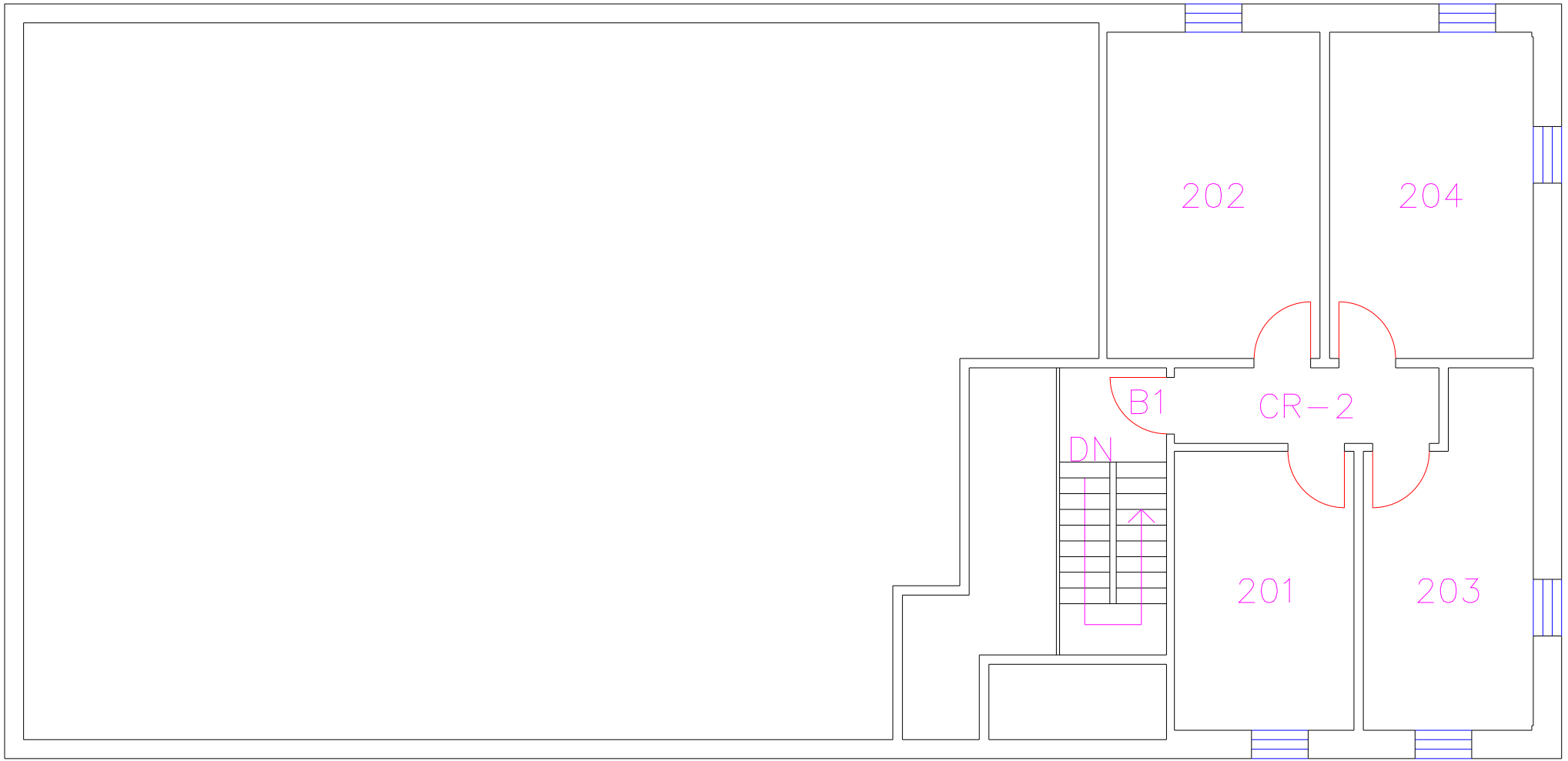
SECOND FLOOR
