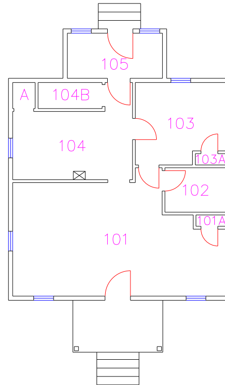
BUILDING 0314
