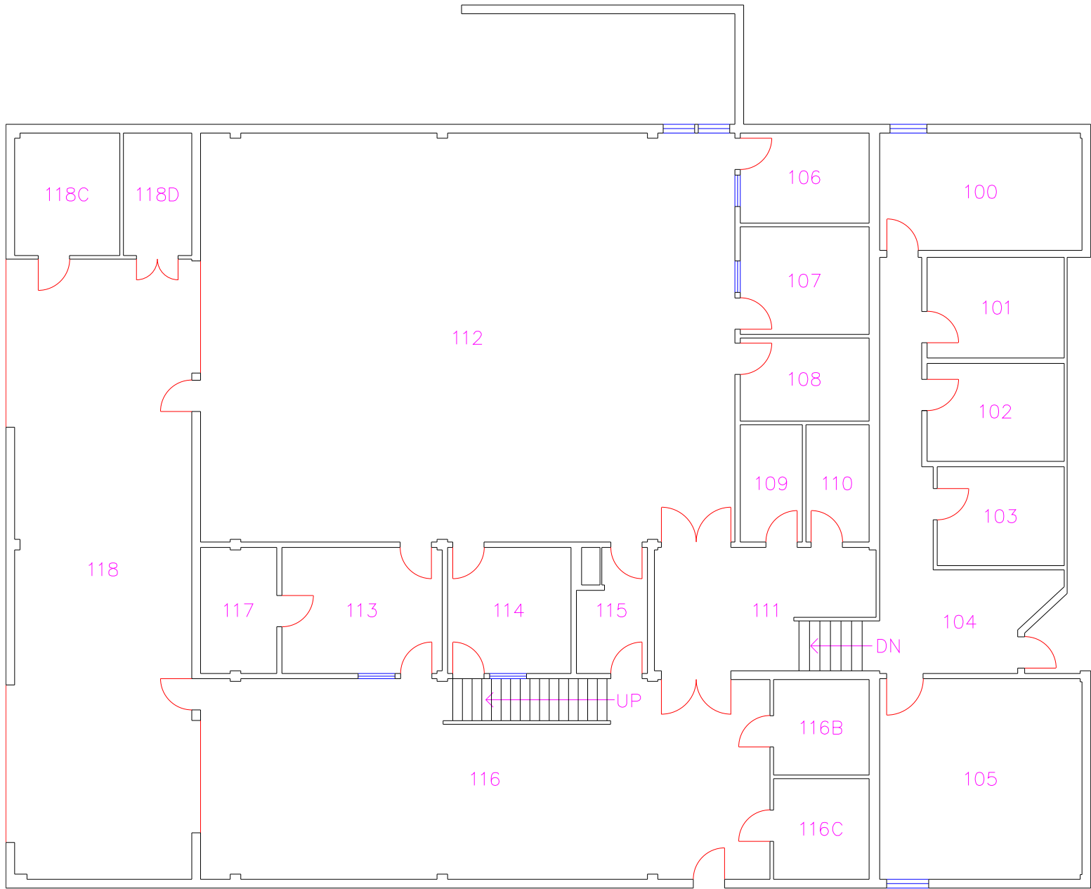
FIRST FLOOR
