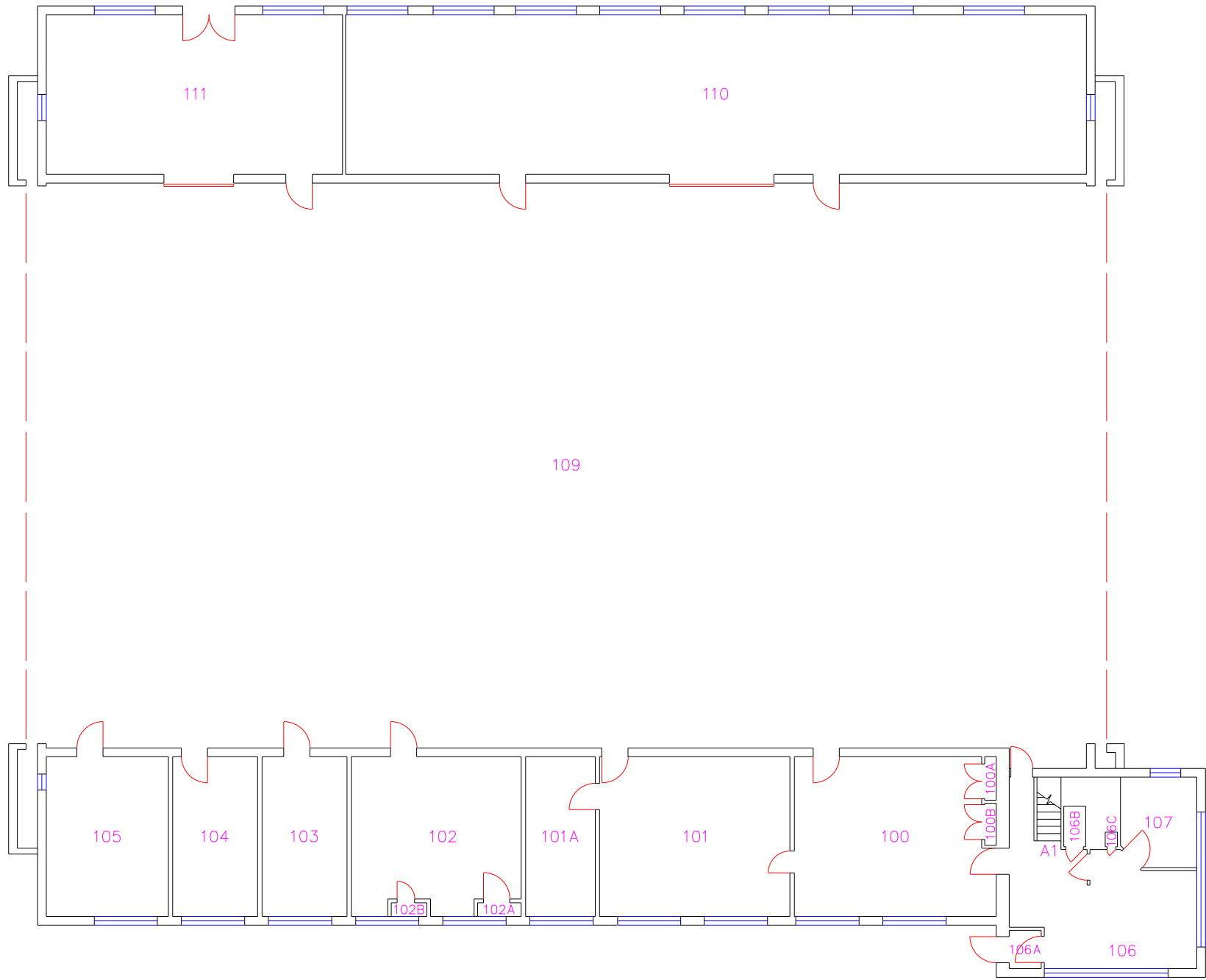
FIRST FLOOR
