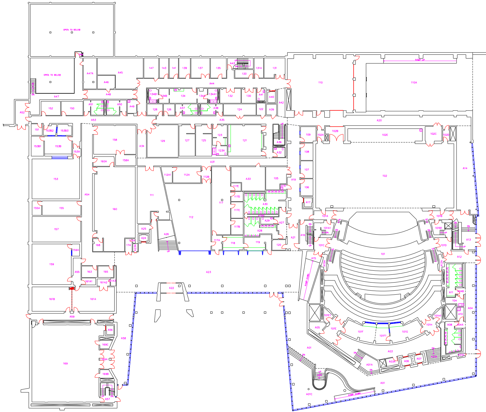
LEVEL 01: FIRST FLOOR
