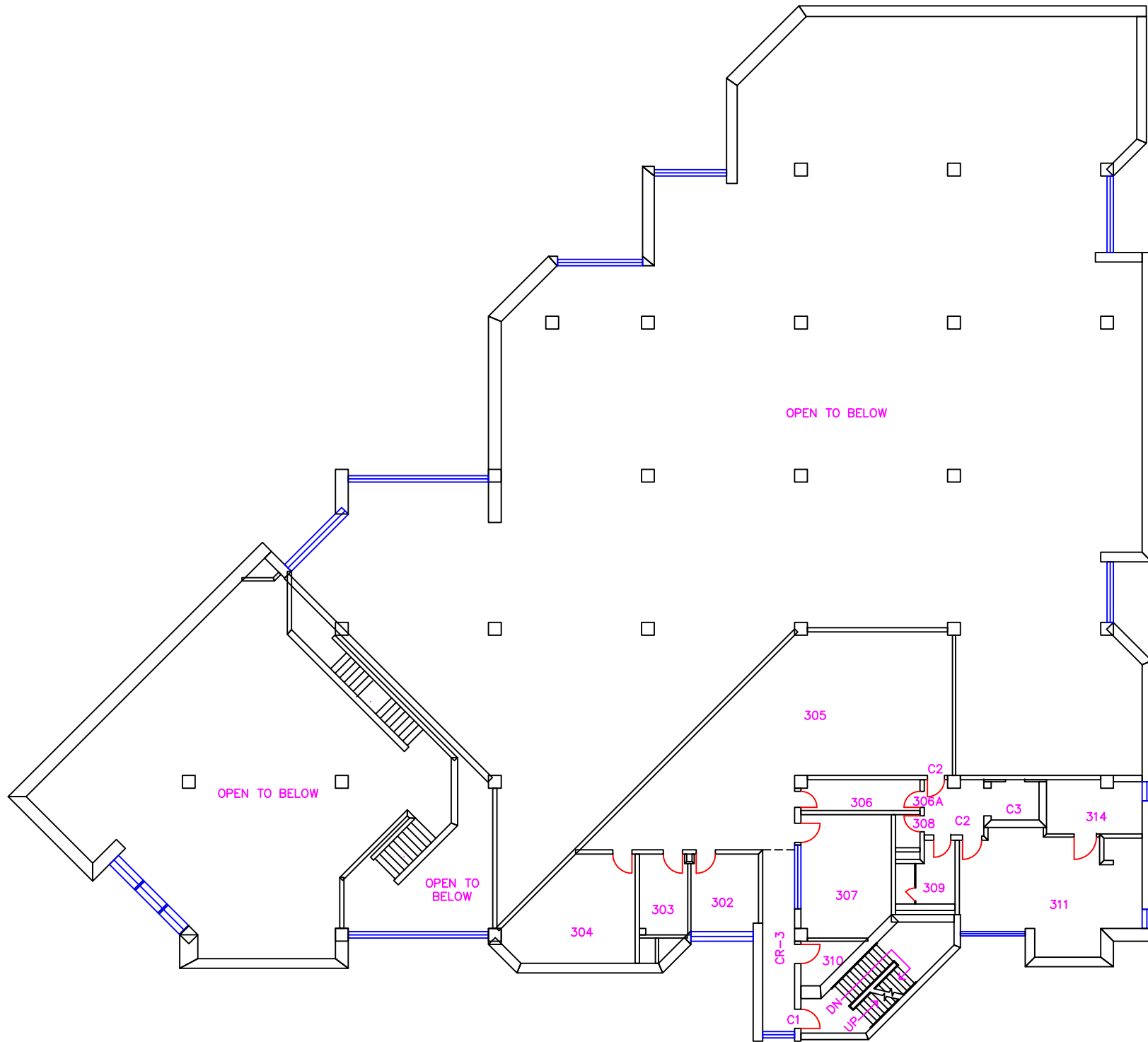
MEZZANINE LEVEL
