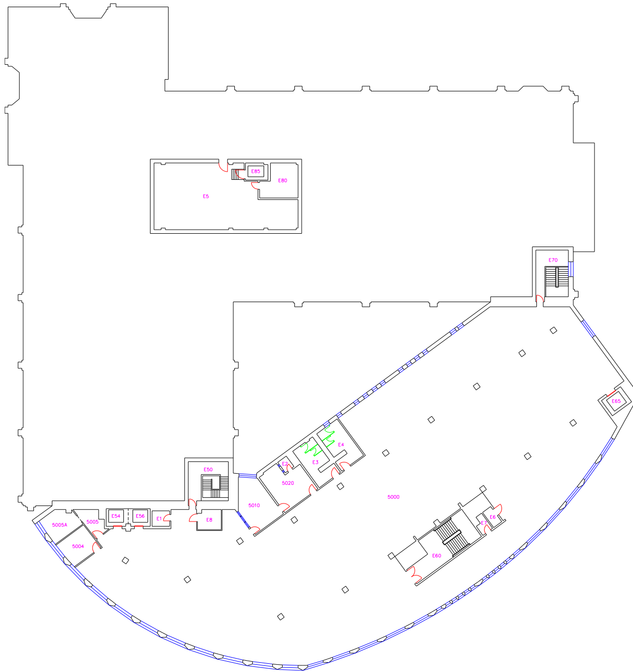
FIFTH FLOOR
