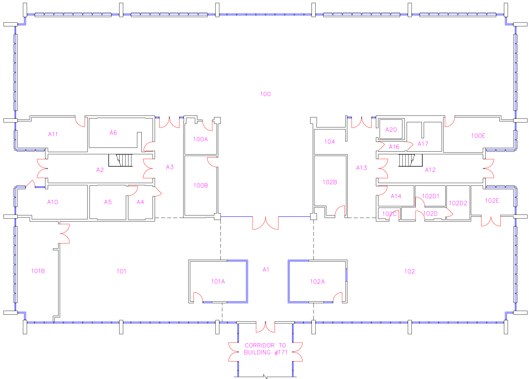
FIRST FLOOR
