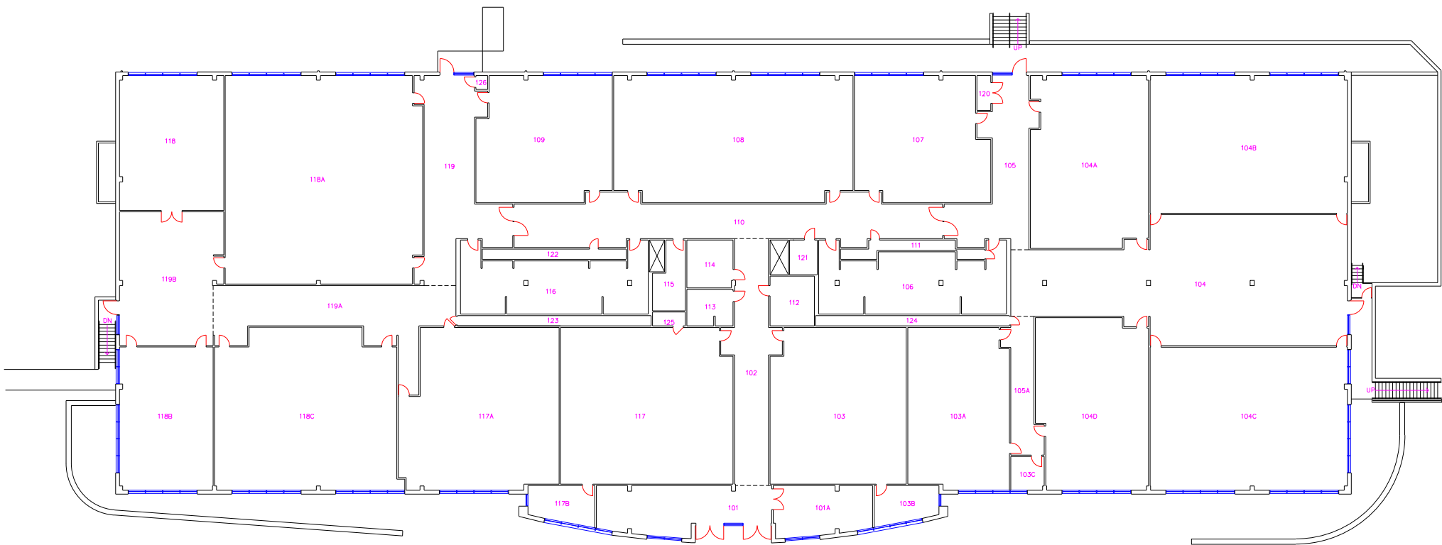
FIRST FLOOR
