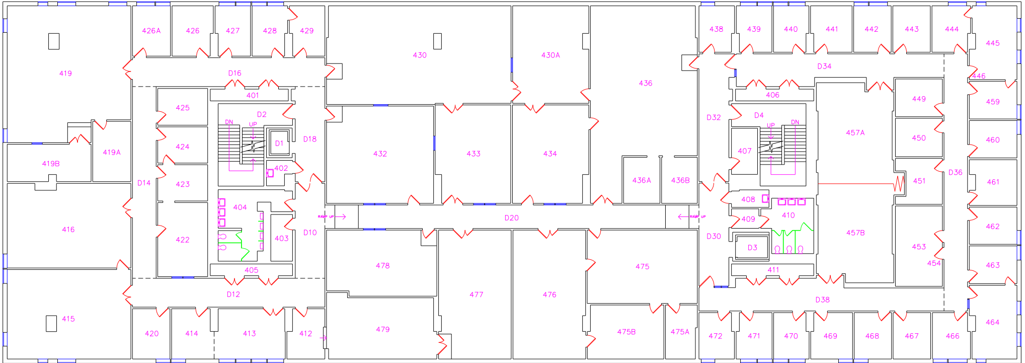
FOURTH FLOOR
