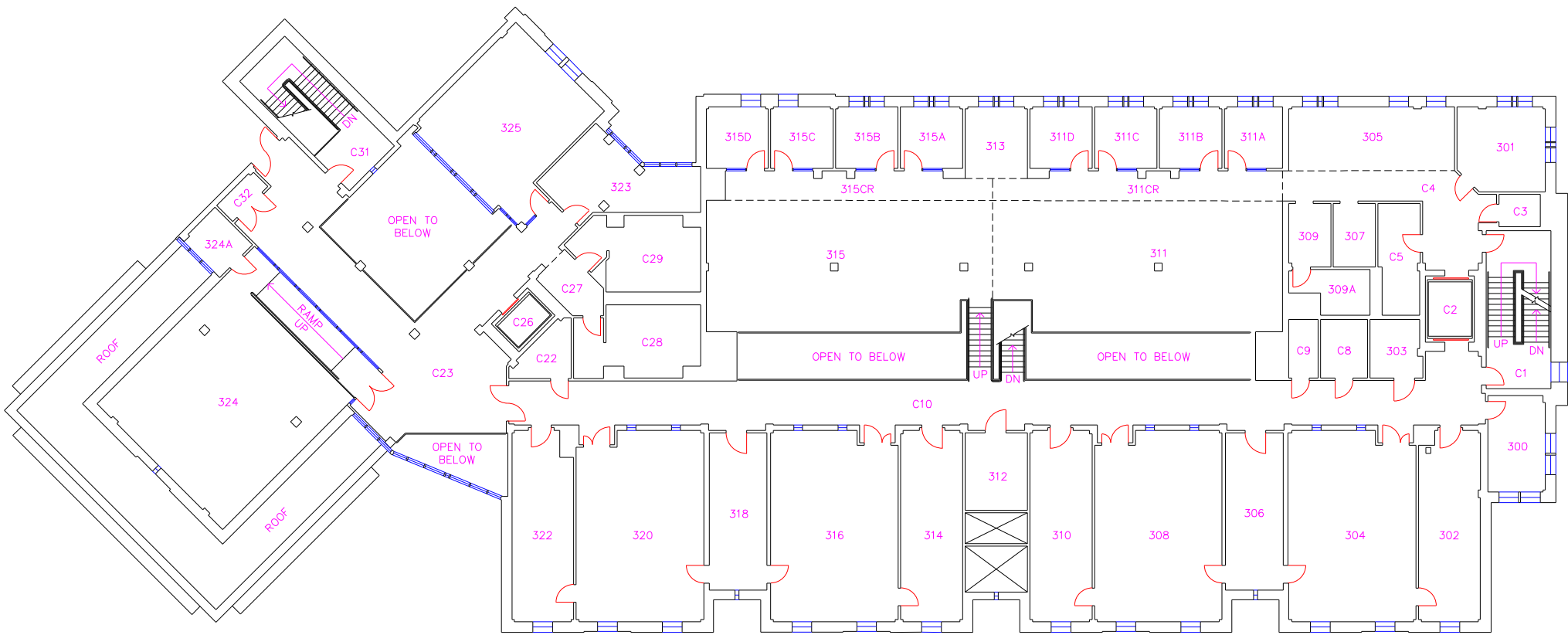
THIRD FLOOR
