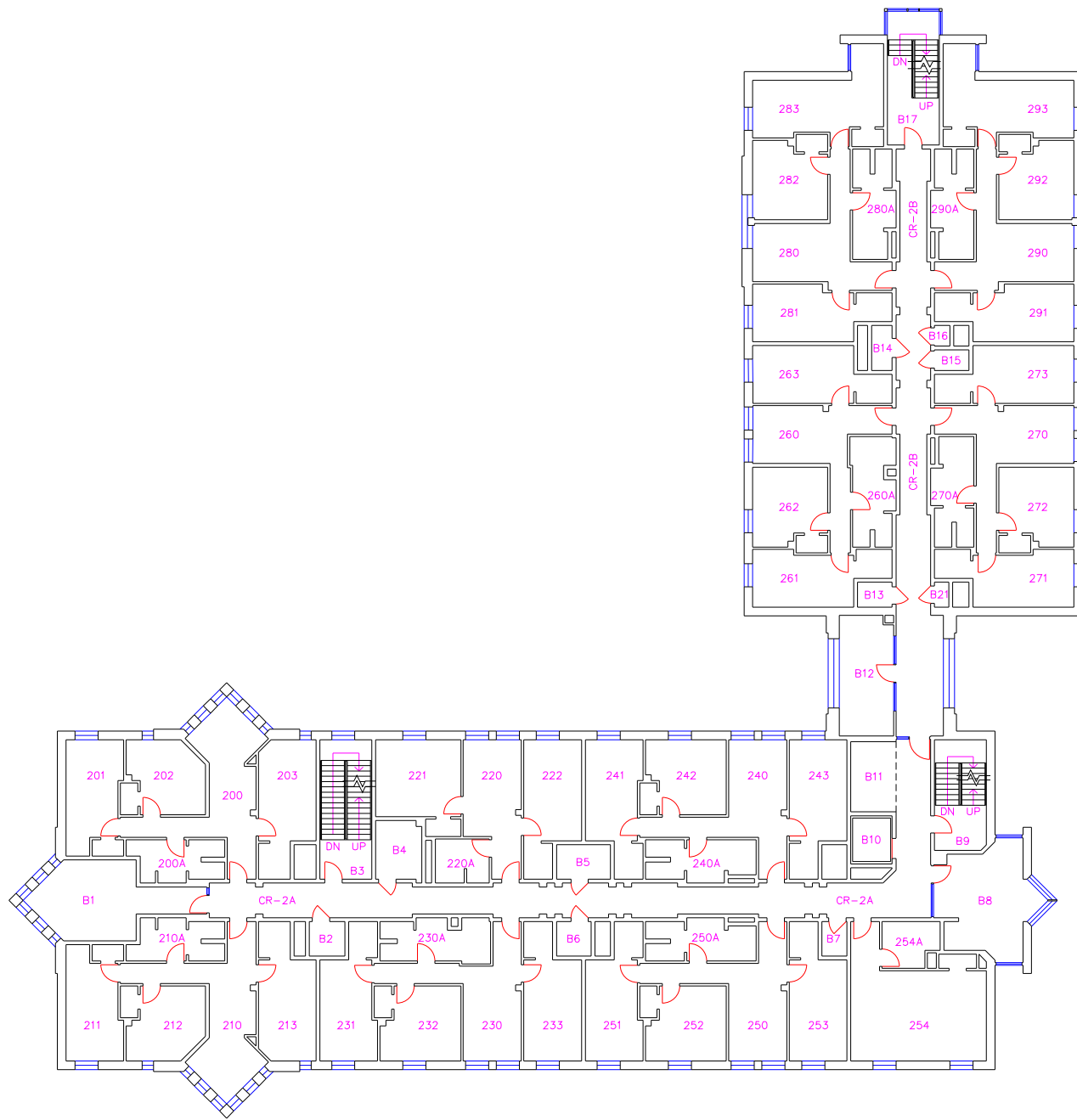
SECOND FLOOR
