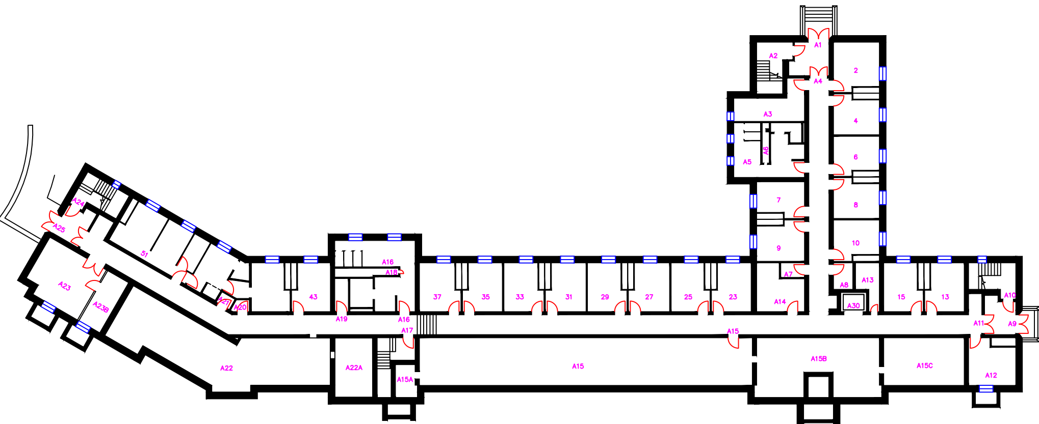
BASEMENT FLOOR
