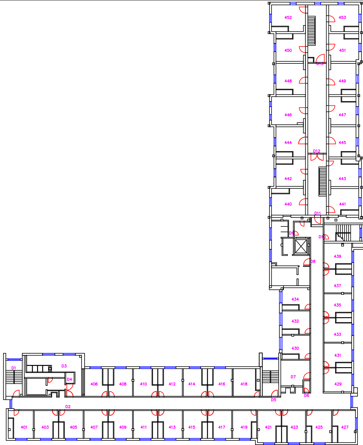
THIRD FLOOR
